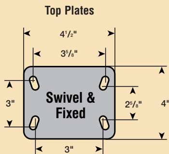
Gang Box Kit top plates are 1/4" thick and have fixing holes to suit 3/8" diameter bolts.
