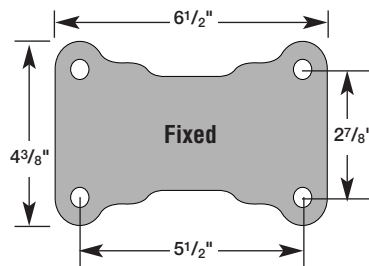
88 Series Casters
