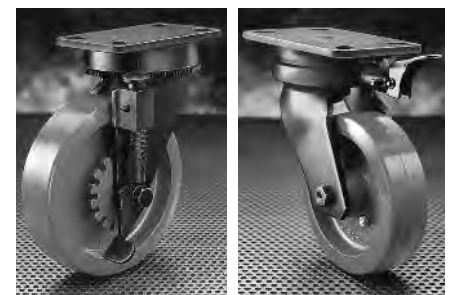
KV Series Swivel & Wheel Brake (8") - Available with Polyurethane-on-Cast-Iron wheel only; add suffix CWL to Swivel Part #.
