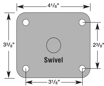
22 Series 4" & 5" Casters
