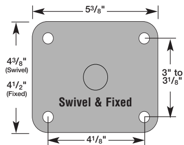
22 & 29 Series 6" & 8" Casters
