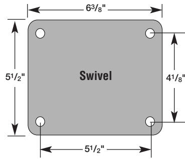
88 Series Casters
