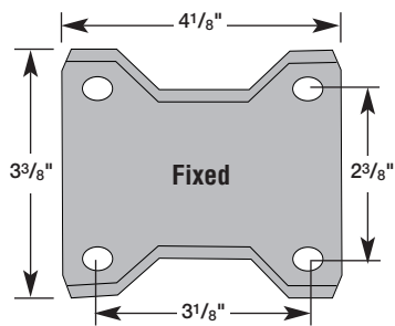
29 Series 4" & 5" Casters
